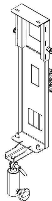
Illustration of Vario system including clamp bracket and tripod mount
